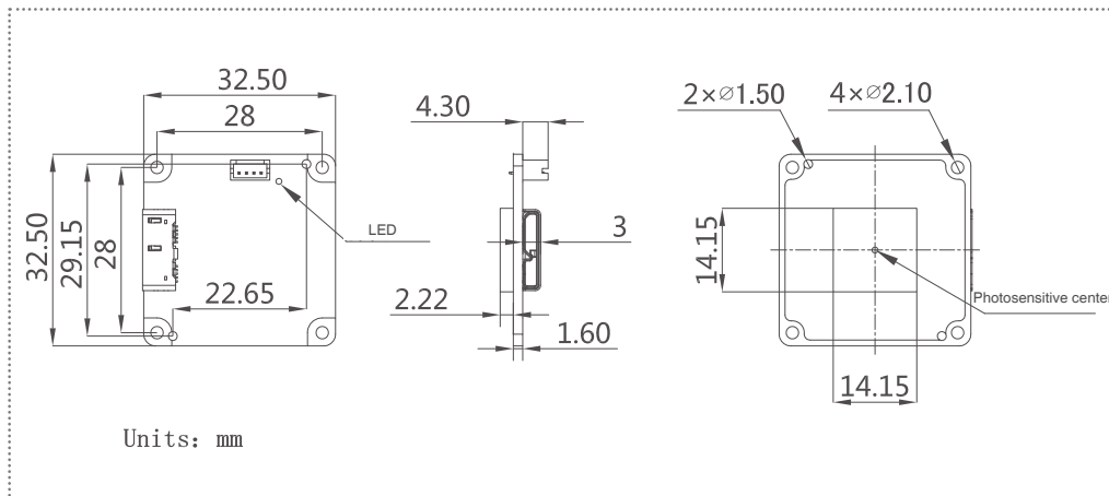
VEN-042-121U3M/C, No-mount
