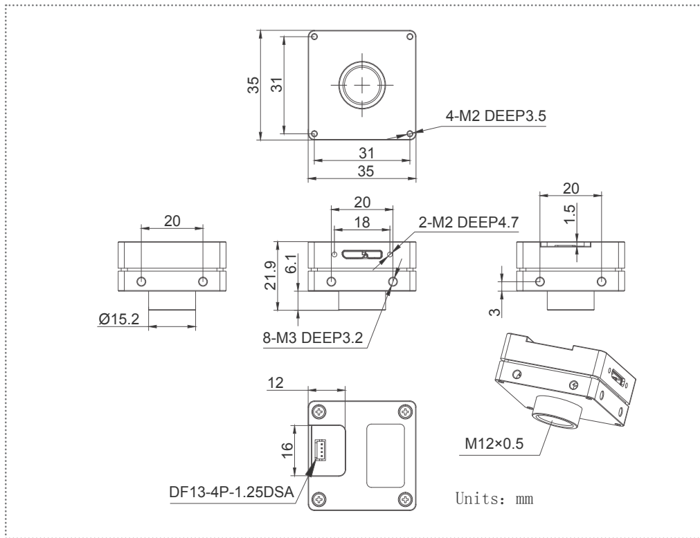
VEN-042-121U3M/C, S-mount
