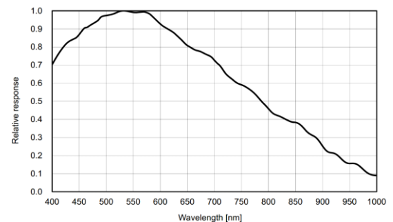
MV-CT*MU0200/R
