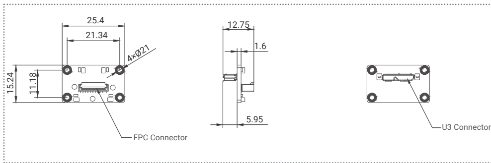
Micro-B adapter board
